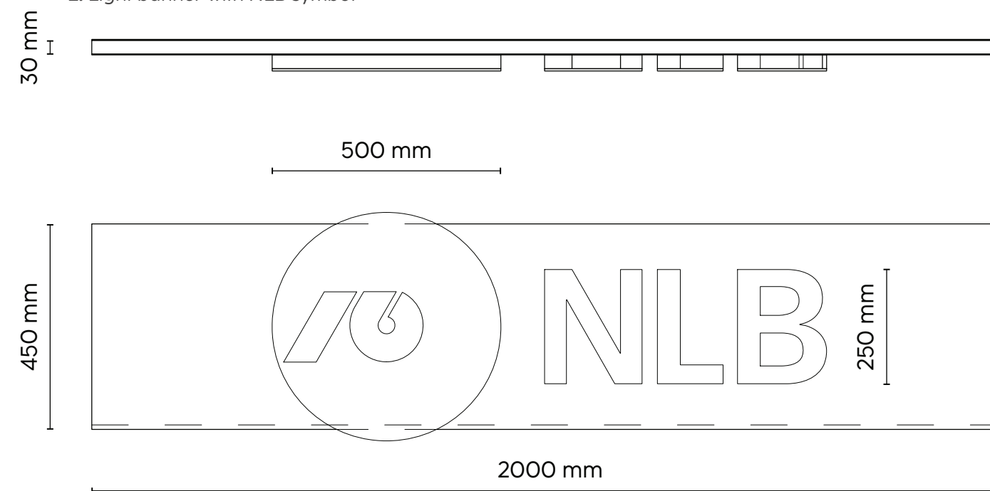
2. Light banner with NLB symbol
